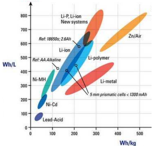
Figure 8 Comparison of batteries in terms of power to weight (x-axis) and power to volume (y-axis)
